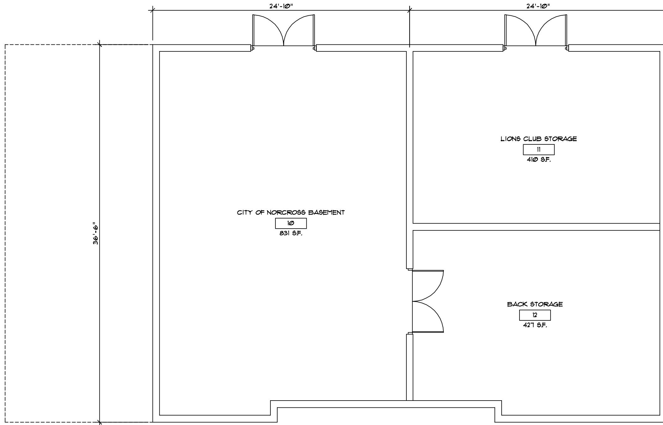
1 PROPOSED BASEMENT LAYOUT A-102 SCALE 3/8" = 1'-0"
