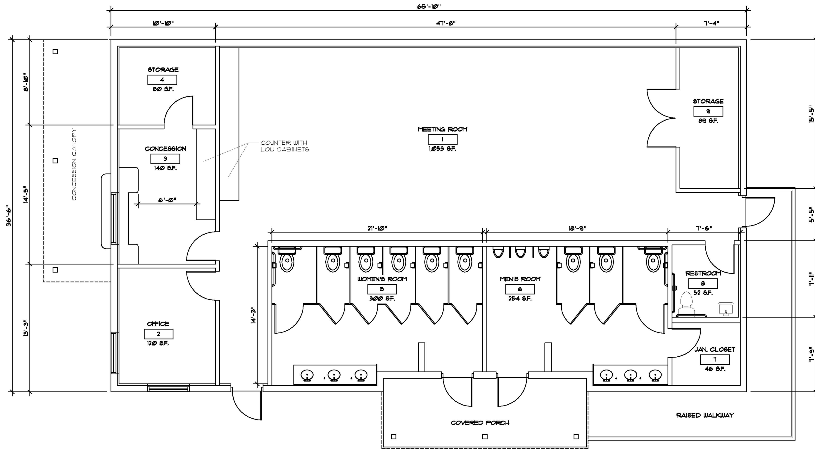
1 NEW BUILDING MAIN LEVEL A-101 SCALE 3/8" = 1'-0" 2,403 TOTAL S.F.
